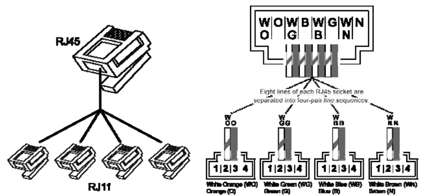
Figure 1-3 Wiring scheme
